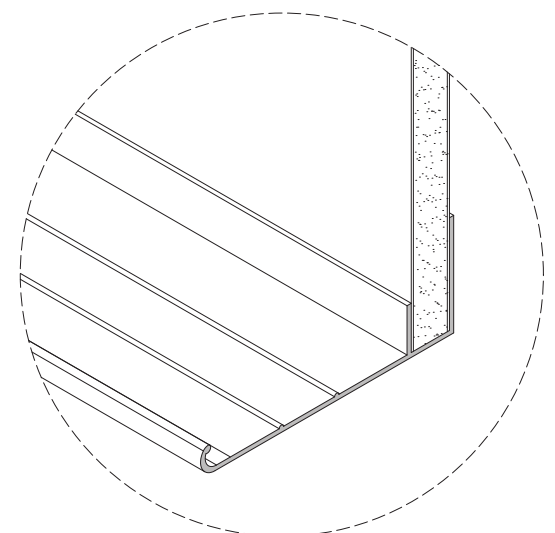
SCREW-ON MARKERTRAY SCALE: 6" = 1'-0"
