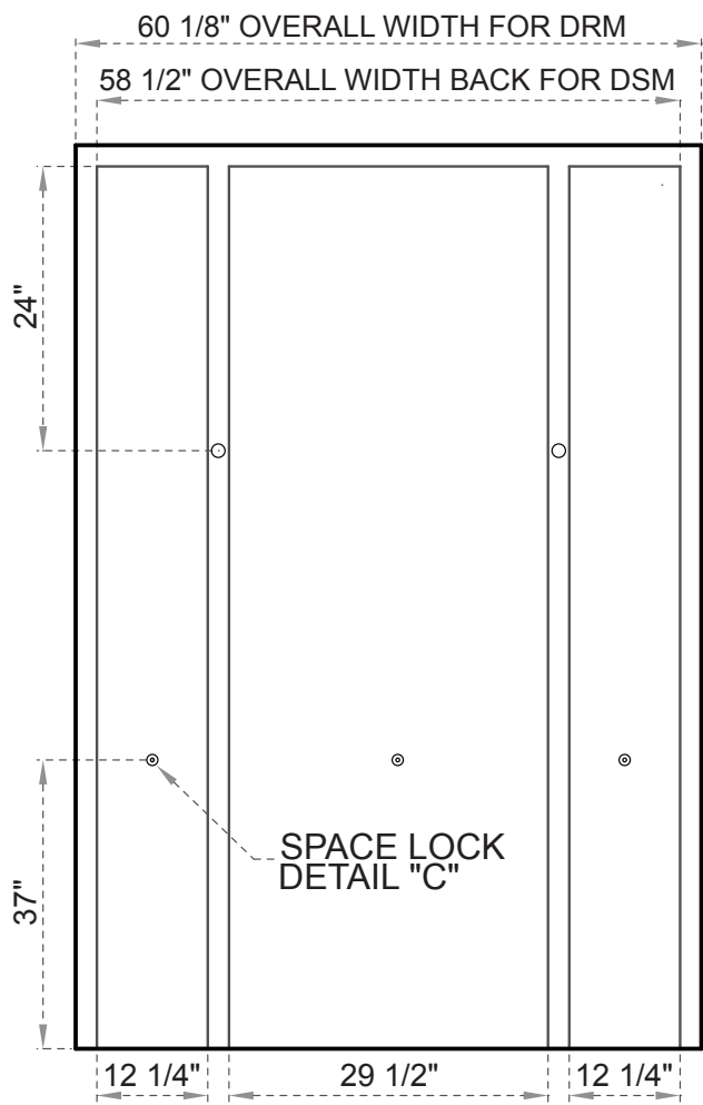
FRONT ELEVATION
