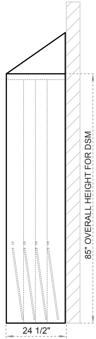
VERTICAL SECTION DSM-12TB MODEL
